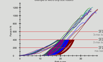
example of Micro Grip test results
